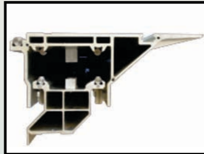
Dual-roller sliding carriage system Smooth running Minimal maintenance
