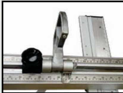
Flip-over stops, with curved base Slide a panel underneath without re-positioning Two adjustable measuring tapes Angled for ease-of-reading
