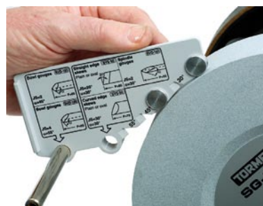
Jig setting distance
